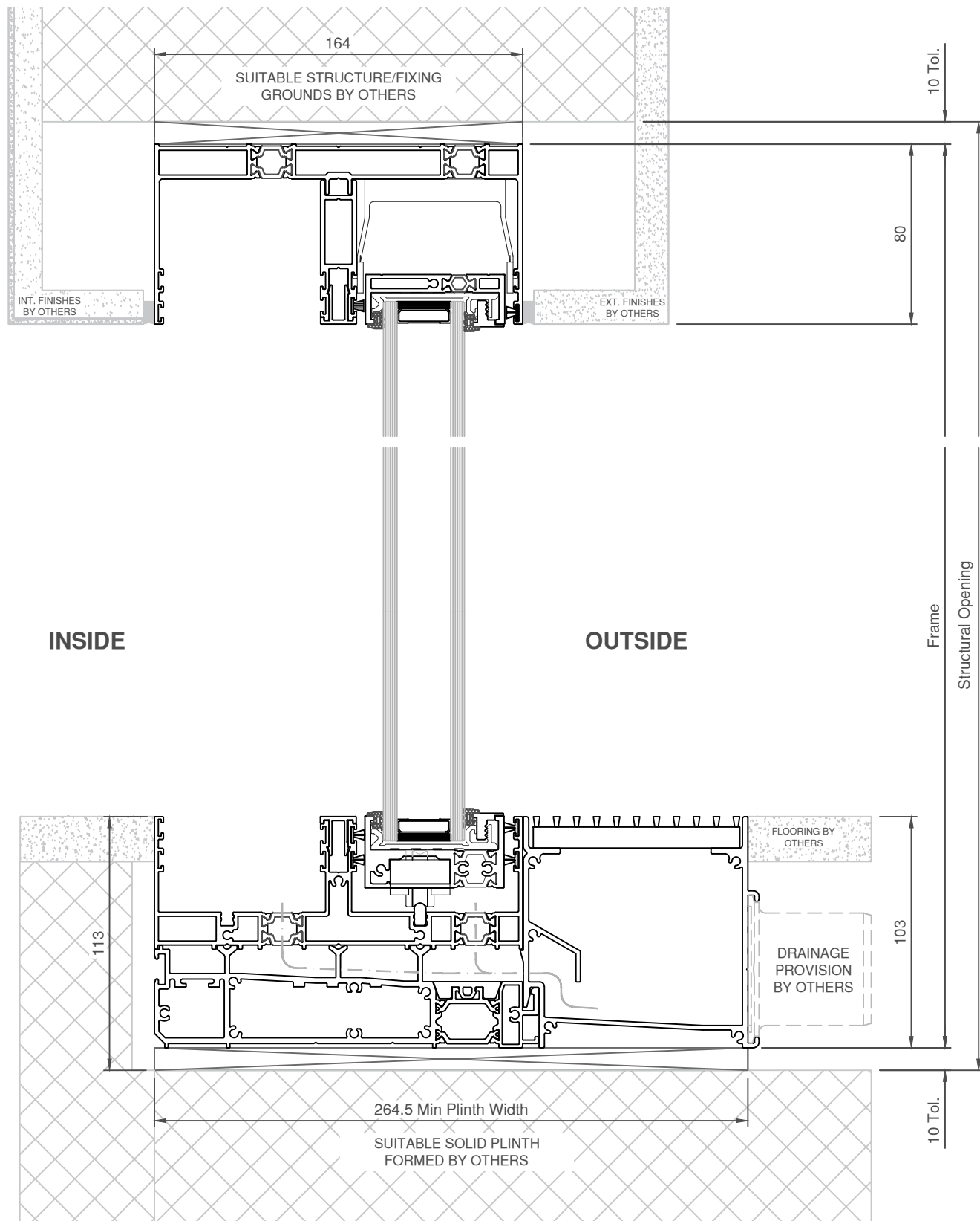
SECTION B-B
