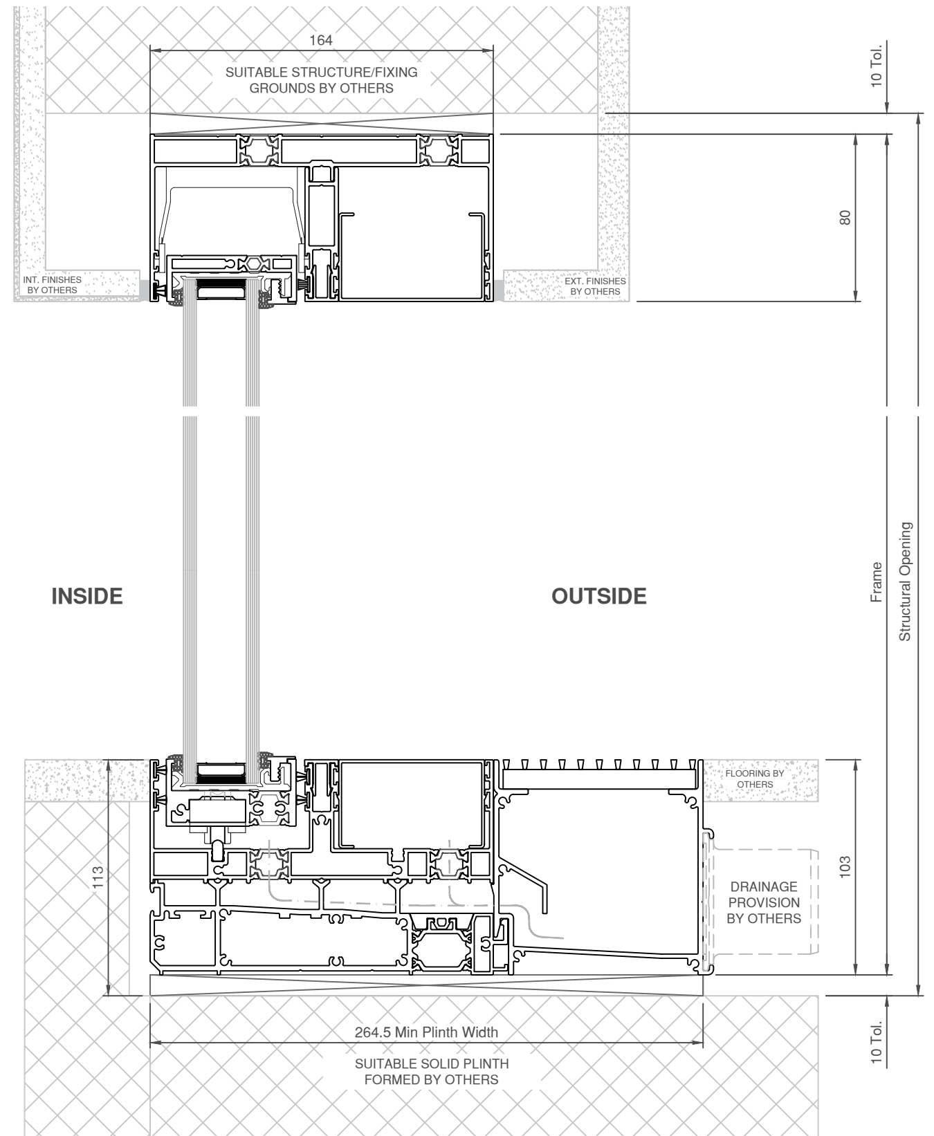
SECTION C-C
